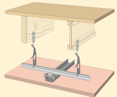
Figure 15: Floor System G
