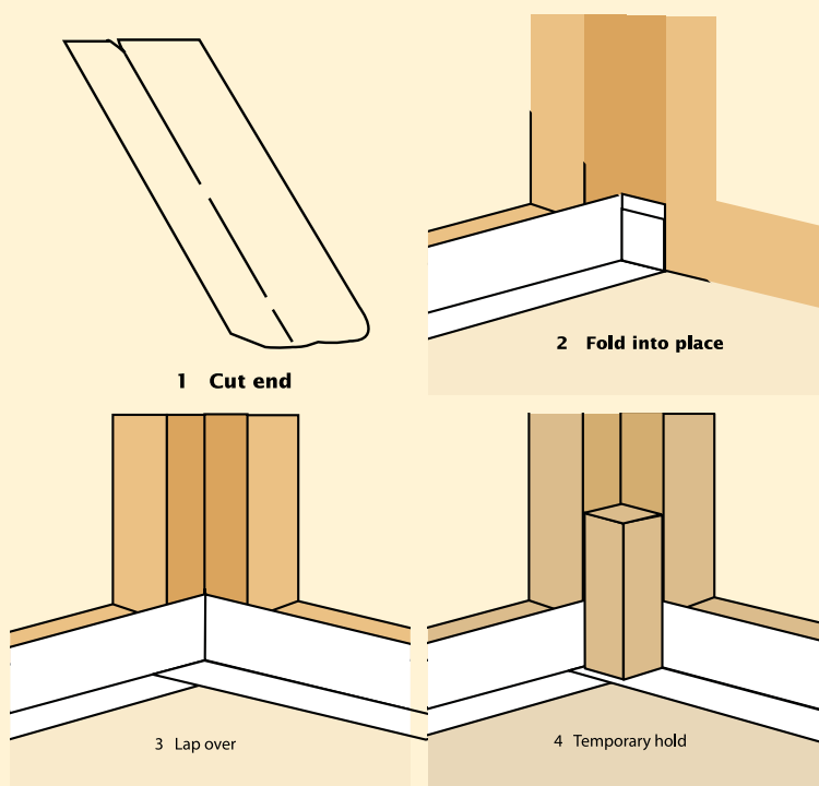
Vertical Flashing
