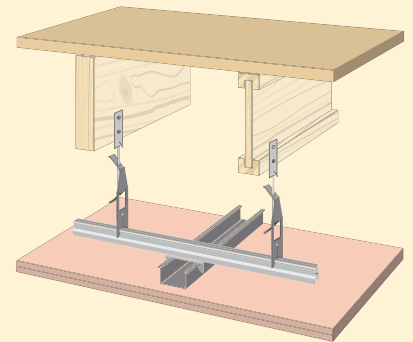
Figure 14: Floor System F
