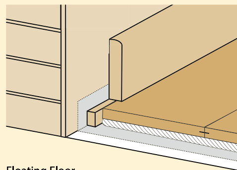
Floating Floor
