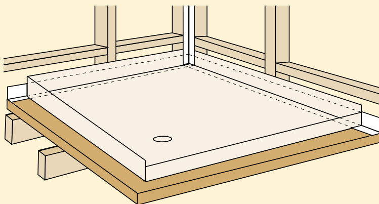
Vertical Flashing
