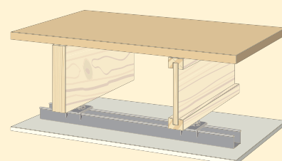
Figure 11: Floor System C
