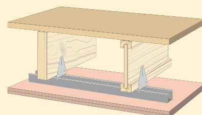
Figure 12: Floor System D
