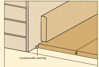
Particleboard flooring on Concrete Loose Laid
