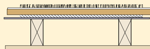
Floating Floor (Over Timber)
