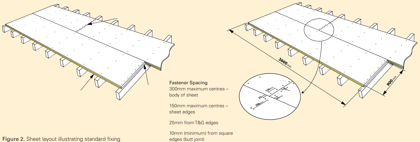
Figure 2. Sheet layout illustrating standard fixing
