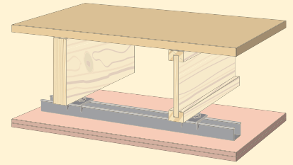
Figure 13: Floor System E
